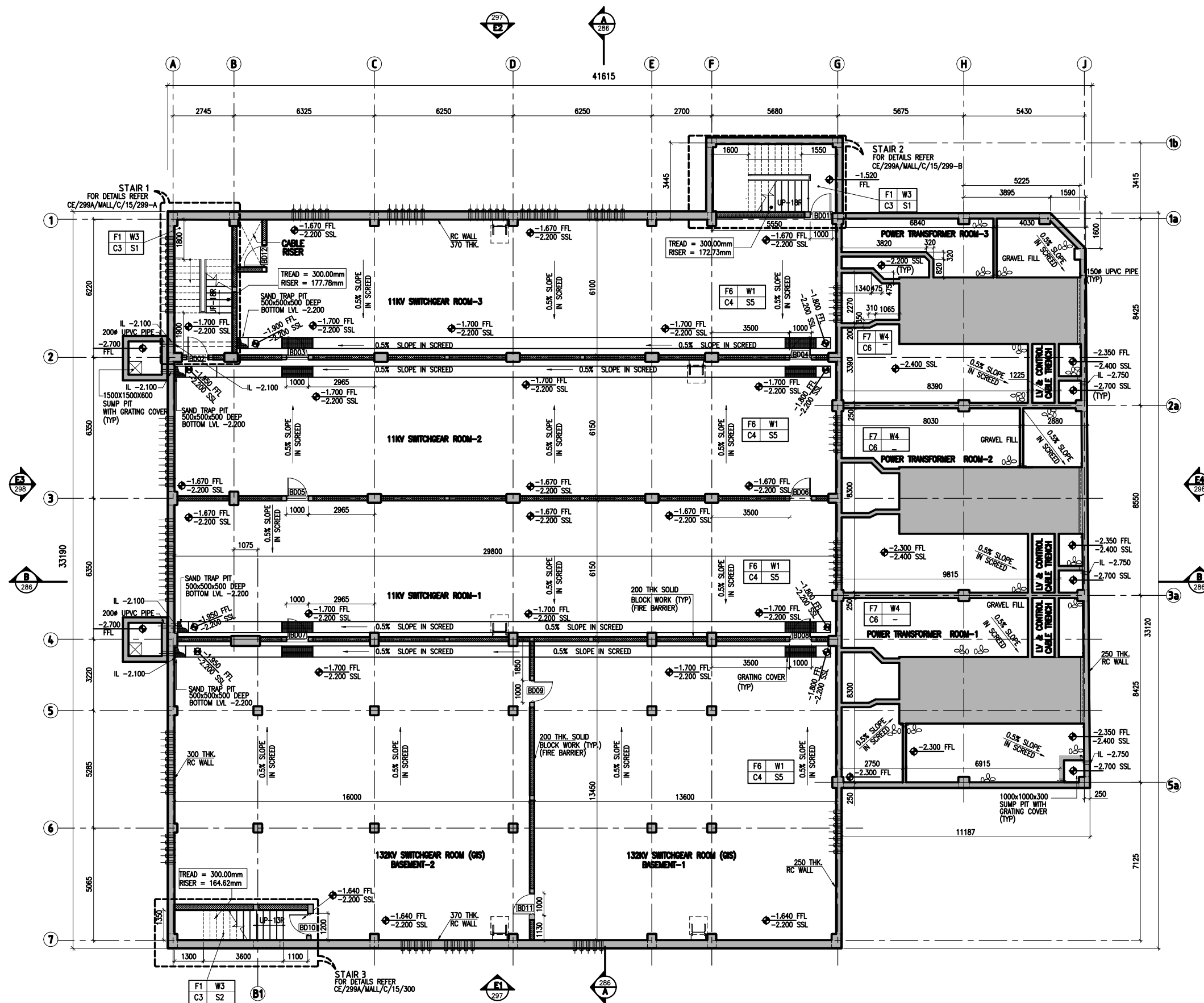
BASEMENT FLOOR PLAN SCALE 1:100
